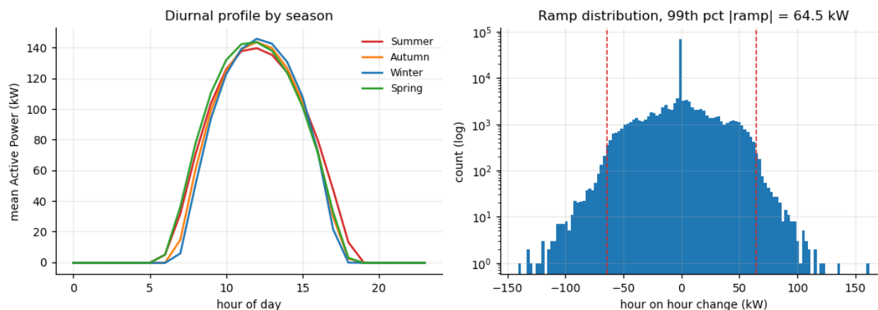
Figure 3. Left: The mean diurnal profile for each season. Right: Distribution of hour on hour change, log scaled, with 99th percentile of absolute ramp at 64.5 kW marked.
