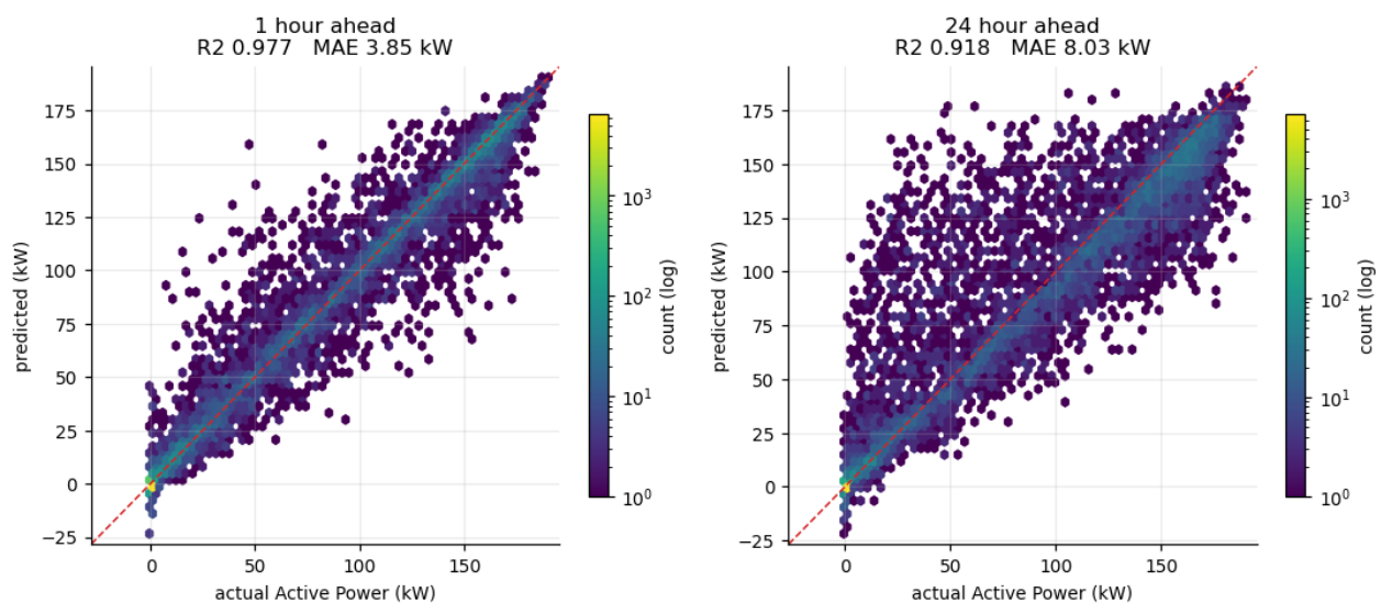
Figure 8. Log-scaled density plotted against predicted. 1 hour model sticks very close to the diagonal. The 24 hour model features the characteristic fan of a forecast without future weather, widest in the mid range where cloud determines the forecast.
