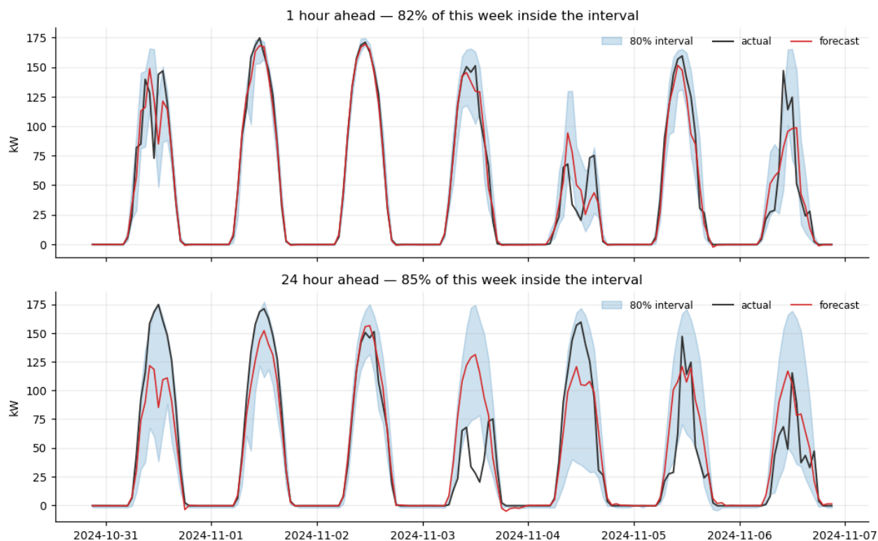
Figure 9A single week of the final fold at the 80% interval shaded. Clear days are tightly forecast at both horizons. On the rough days of 3rd and 4th November the interval is expanded such that it is easily seen by the operator.
