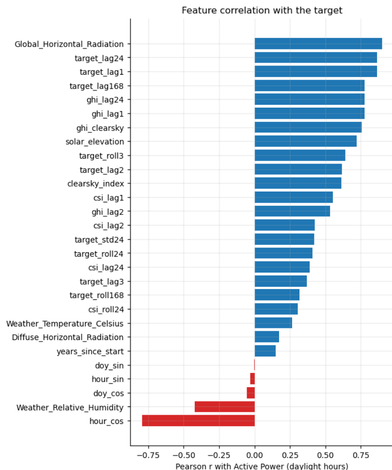
Figure 4. Pearson correlation for all features and the target (day light hours only). The night is omitted because there is no information to be gained from a correlation that has a common zero at night.
