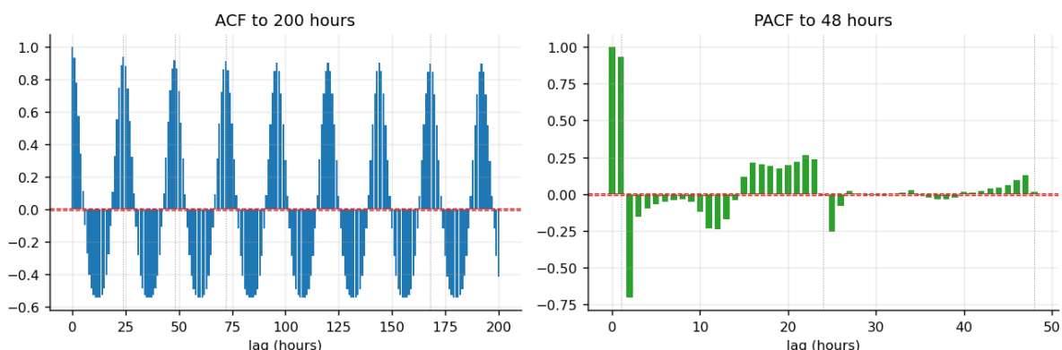
Figure 6. An AutoCorrelation and Partial AutoCorrelation of Active Power computed on the complete hourly grid with time aware shift; thus, lag k is exactly k hours. The ACF peaks at multiples of 24 confirm the presence of the daily cycle in the data, and the PACF indicates which shorter lags contain information not already included in the other lags and justifies the use of the 24 and 168 hour lags.
