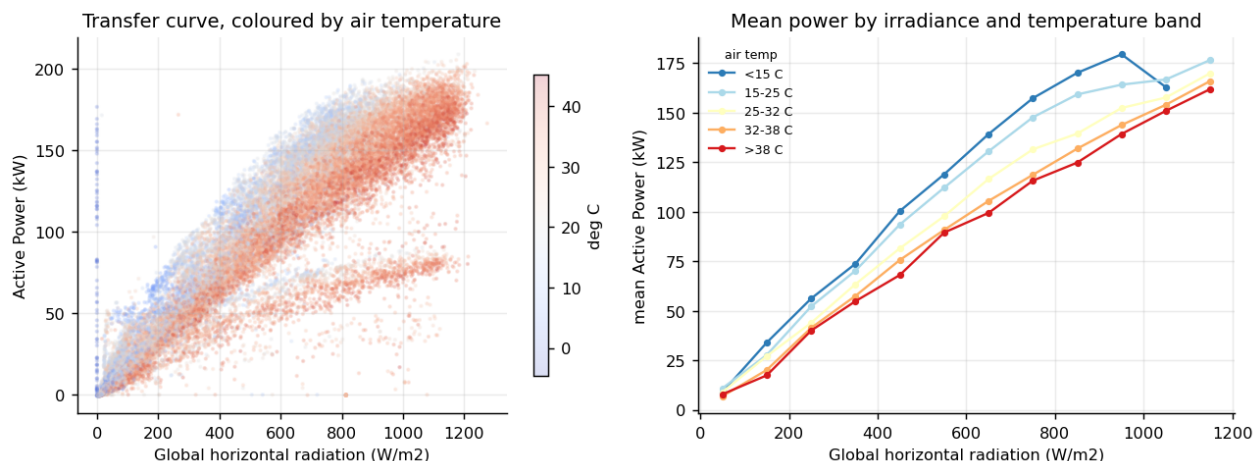
Figure 7. Left the physical transfer curve in color according to the temperature of the air. Right: Irradiance band averaged mean power as a function of temperature band.
