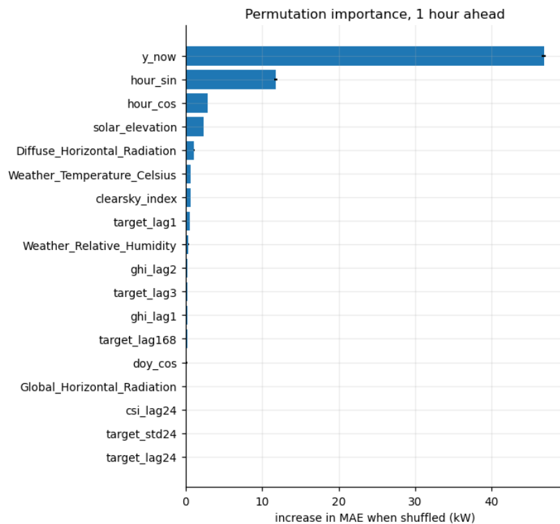
Figure 10. The permutation importance at 1 hour horizon (how much MAE is increased when a feature is shuffled). This is unlike split counts as it shows the impact on the held out performance.
