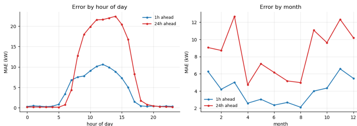
Figure 11. Mean absolute error for each hour of day and each month. All the error is almost totally concentrated in the daylight: 6.77 kW against 0.40 kW at night for the 1 hour model, 14.62 kW against 0.26 kW at 24 hours.
