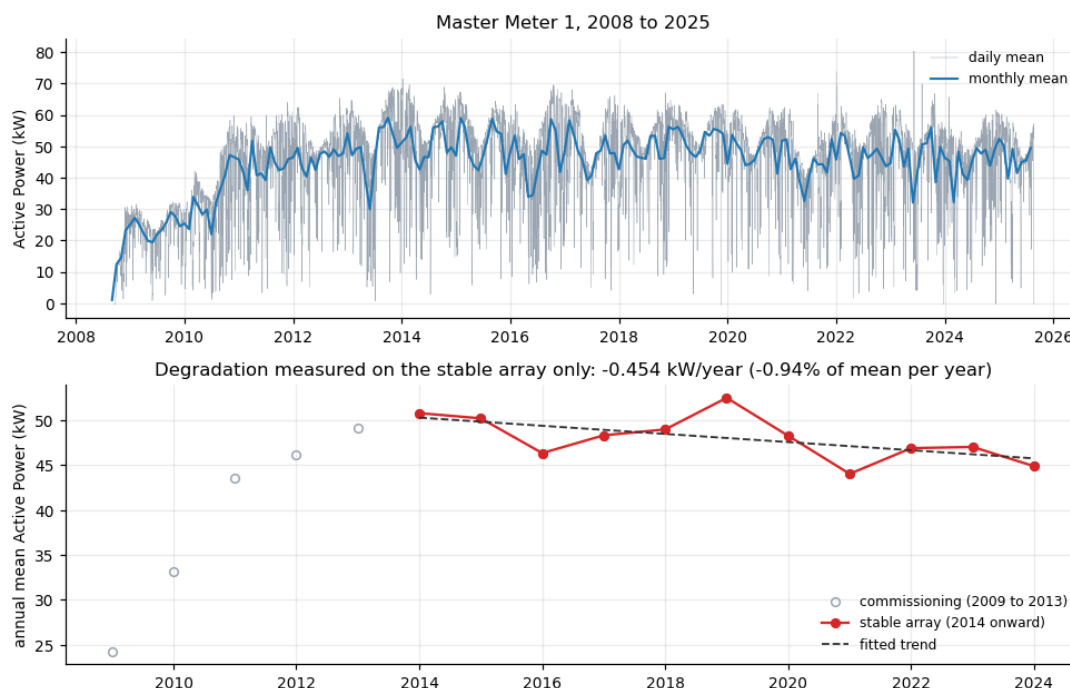
Figure 2. 17 years of Master Meter 1 production. Upper: Daily mean (grey) and monthly mean (blue). Lower: annual means (open markers indicate 2009–2013 commissioning period; only fit from 2014).
